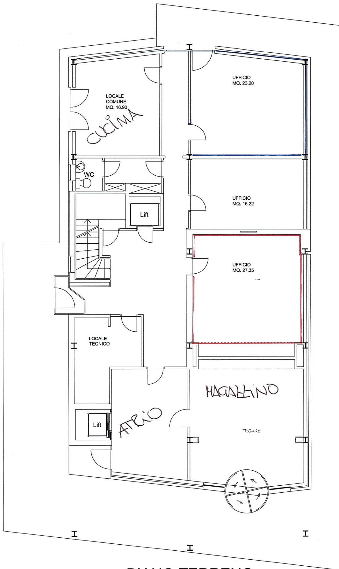
PIANO TERRENO
